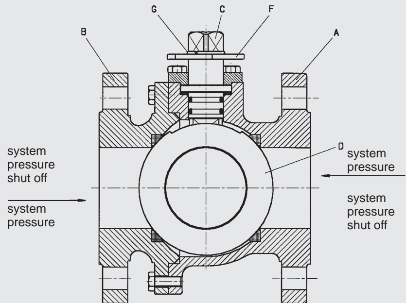
Ball valve closed
