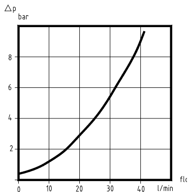
Anticavitation characteristics TBSD121 and SB160
