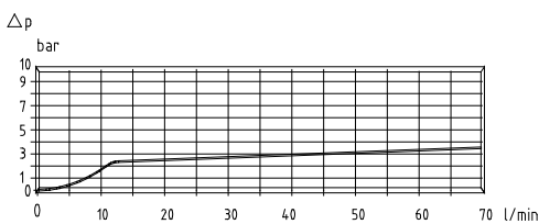
Pressure drop P1 - T4, inlet I02Q/I06Q, unloaded
