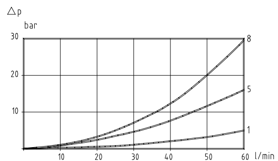
Pressure drop, P1 - T1/T3, inlet I02C, outlet U01B
