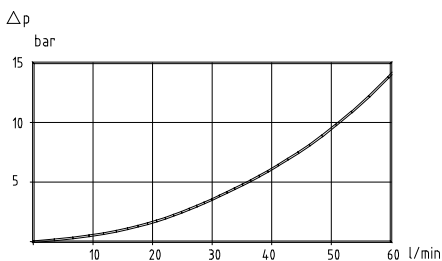
Pressure drop, P1 - T4, inlet I01E, unloaded
