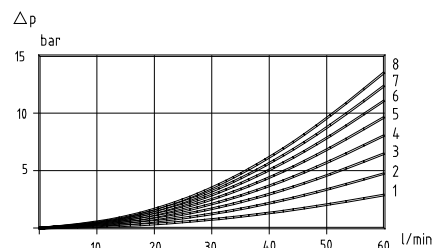
Pressure drop, P1 - T1/T3, inlet I01E, outlet U01B
