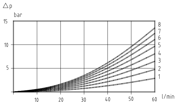
Pressure drop, P1 - T4, inlet i02C, outlet U01C
