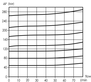
Pressure drop characteristics TBD/TBSD121
