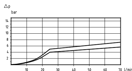
Pressure drop, P1 -T4, inlet I02Q/I06Q, with flow control FKA283/2 and PF12, outlet U01B
