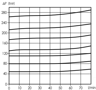
Relief characteristics TBD/TBSD160
