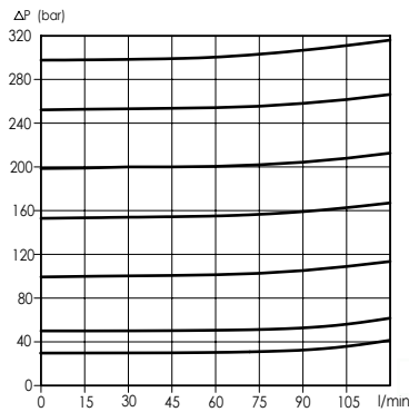
Relief characteristics TBS400
