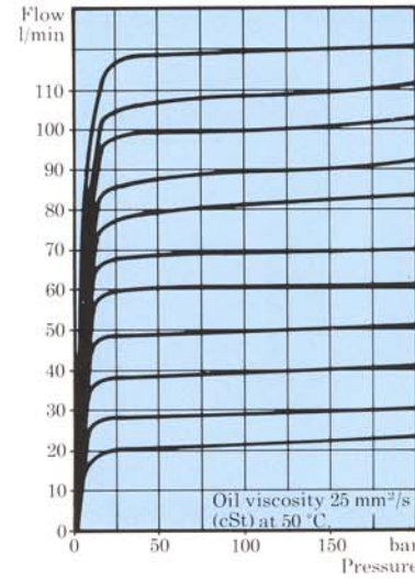
Flow characteristics FKA 332
