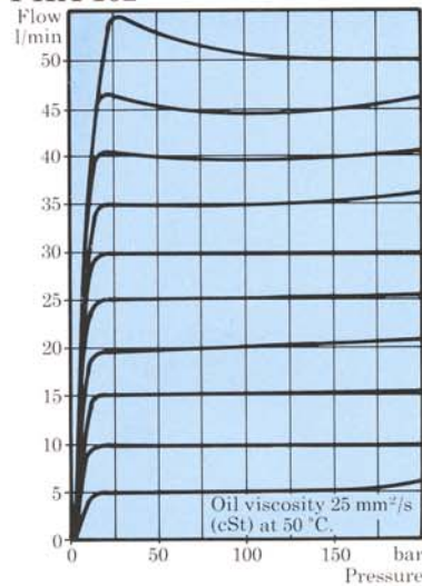
Flow characteristics FKA 162
